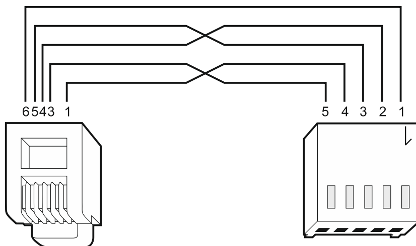
Fig. 3. Wiring diagram of the cable connecting RS-232 ports of INT-GSM module and INTEGRA / INTEGRA Plus control panel with RJ type connector socket.
